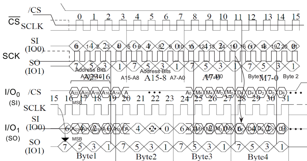
Figure 6-5. Dual-I/O Read Array (Previous command set M5, M4 = 1,0)
